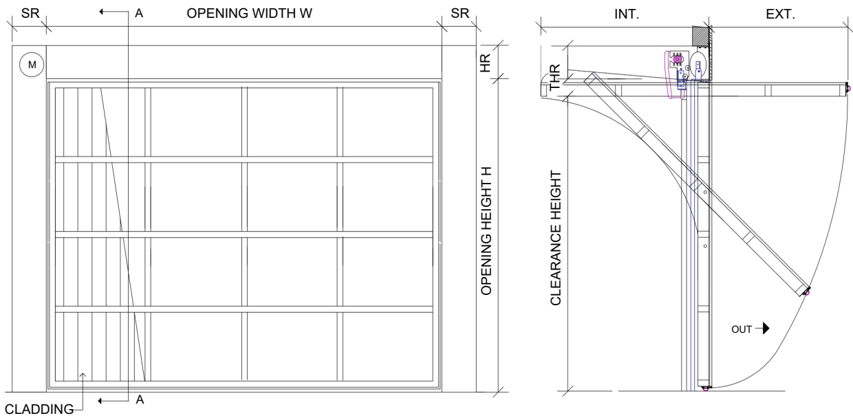
INT. ELEV: INDICATIVE ONLY: FACADE GARAGE DOOR - TILT: type SLE DRAWN SECTION VIEW A- A
