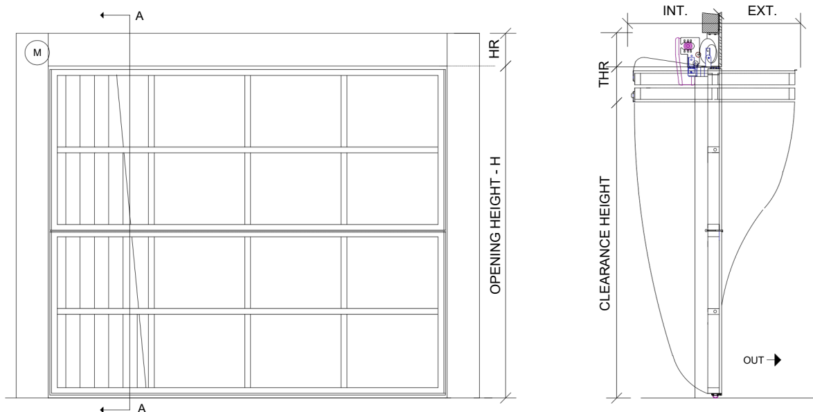
INT. ELEV: INDICATIVE ONLY: FACADE GARAGE DOOR - FOLDING: type SLE DRAWN SECTION VIEW A- A
