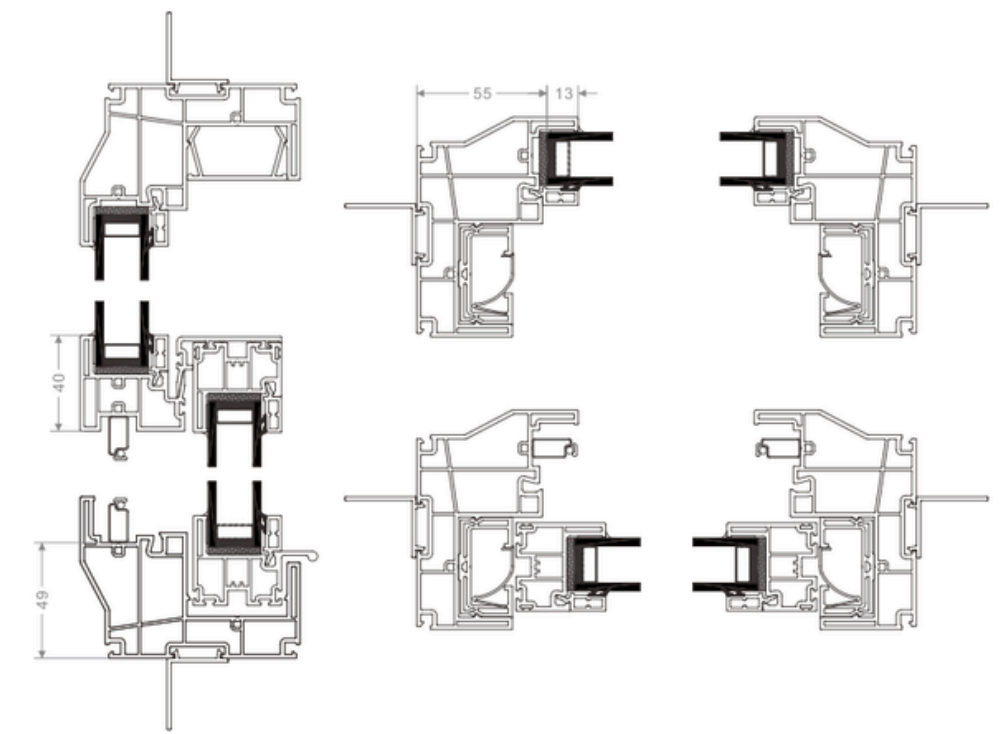
Vertical view
