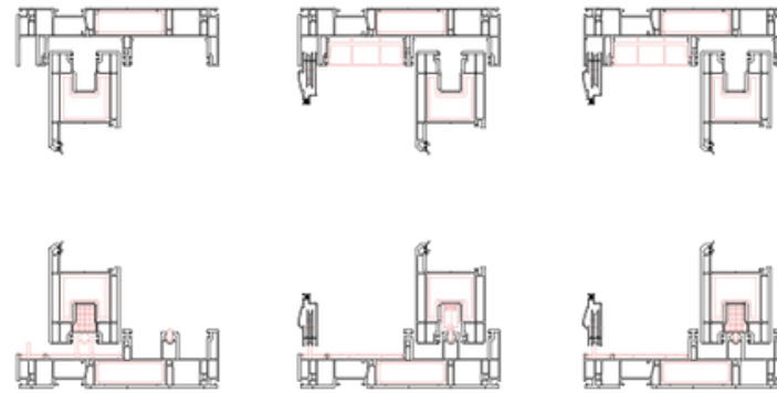
Vertical view
