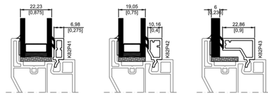
Frame Glazing Bead
